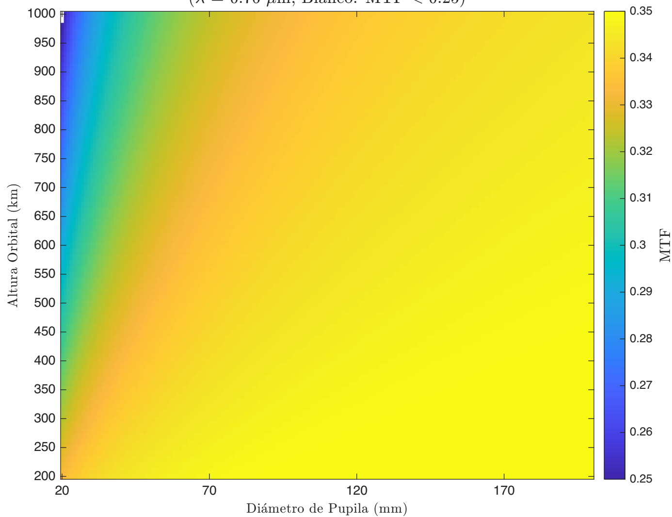
MTF - Refractivo - Detector 1 ( \lambda = 0.76 \mu\text{m} , Blanco: MTF < 0.25)
